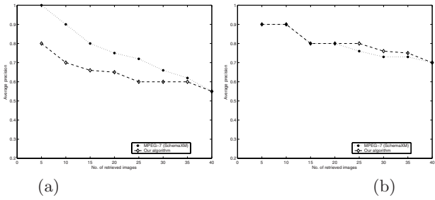
Fig. 4. Comparison with MPEG-7 visual descriptors (a) Category beaches (b) Flowers
