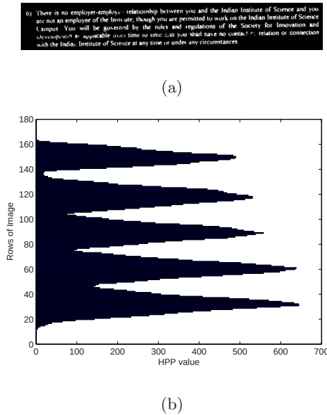
Fig. 2. (a) Example of a typically skewed block (b) HPP of the skewed block
