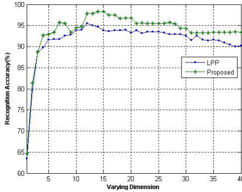
Fig. 2. Recognition accuracy for varying dimensions
