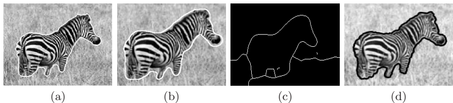
Fig. 5. Comparative study of results: (a) reproduced from [12], (b) reproduced from [13], (c) obtained using the method presented in [14], (d) proposed technique
