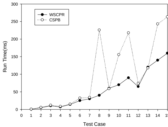
Fig. 1. Performance comparison between WSCP and CSPB algorithm
