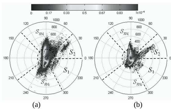
Fig. 4. Histograms in the Polar coordinate system of (a) X_D^0 and (b) X_D^4
