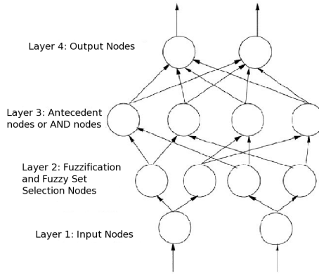
Fig. 1. The network structure for classification
