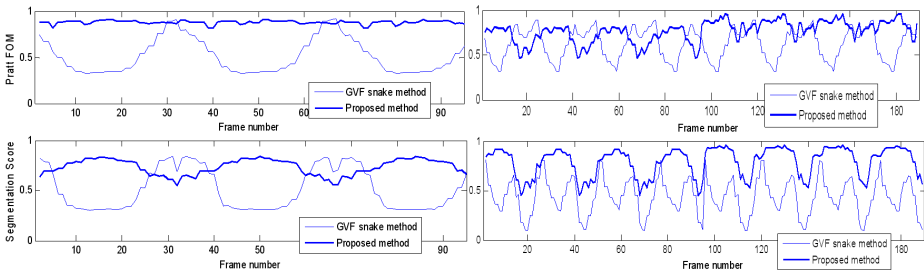
Fig. 3. Comparison of segmentation metrics for GVF snake method and the proposed method on the BSL (left column) and the PK (right column) sequence
