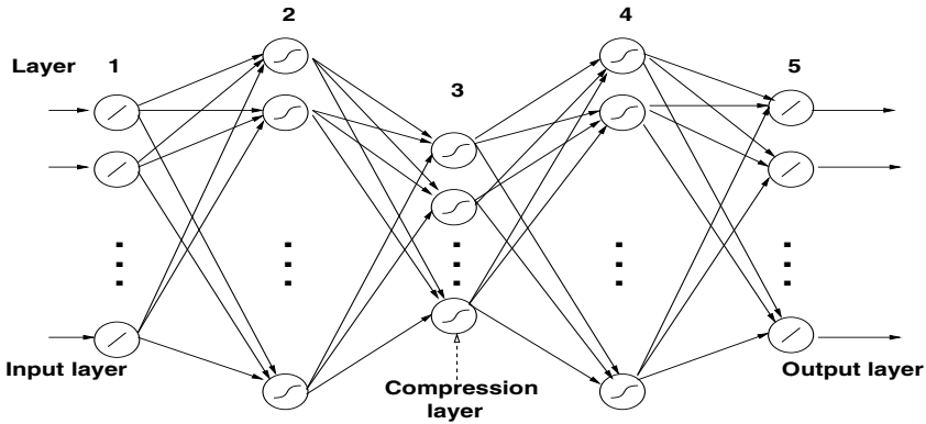
Fig. 1. A five layer FFNN model
