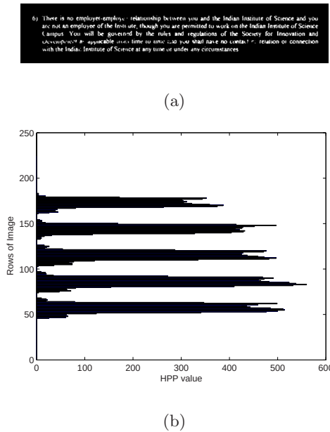
Fig. 1. (a) Example of a typical correctly oriented block. (b) HPP of the correctly oriented block.
