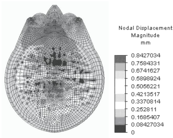
Fig. 3. FEM modeling. Nodal displacement. A head of a child under diffused 120 kg blow on the left brain side.
