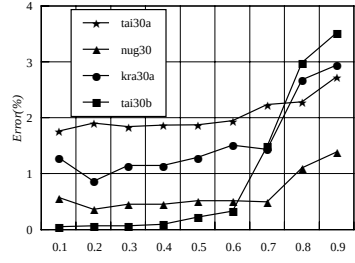
Fig. 2. Change of Error of cAS without local search for various \gamma
