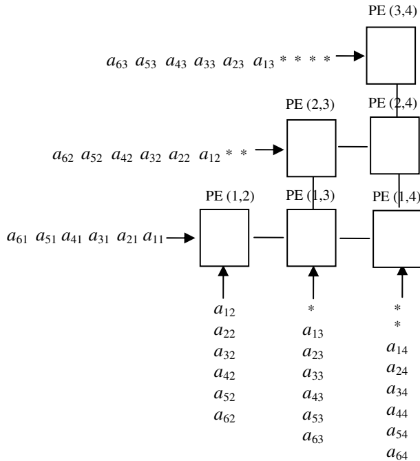
Fig. 3. Triangular array for computing the conflict graph of 6×4 matrix
