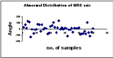
Fig. 4. Abnormal distribution of QRS axis
