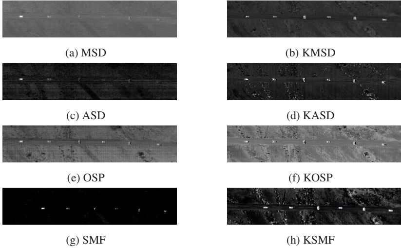
Fig. 2. Detection results for the DR-II image using the conventional detectors and the corresponding kernel versions
