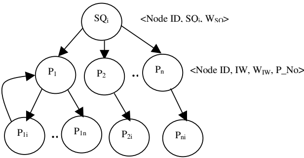
Fig. 1. User's Search Behavior (USB) graph
