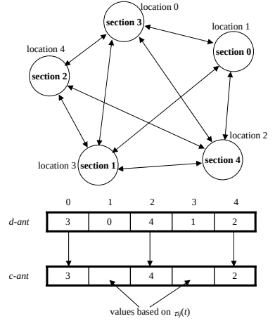
Fig. 1. c-ant and d-ant in QAP
