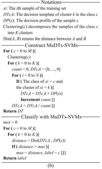
Fig. 3. (a) An overview of MuDTs method, (b) the pseudo code
